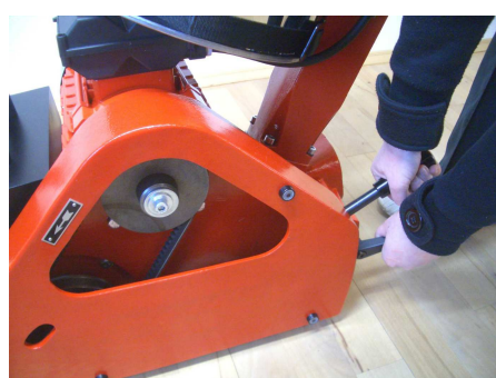
Tightening of the V-belt
